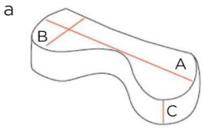
Neck Cushion: 0319-7001-000 A Length 36 cm B Width 6.5 cm C Height 10 cm
